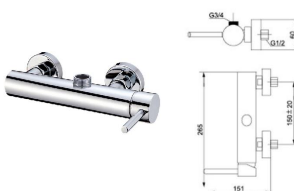
Monomando toma superior 3/4 para kit ducha. Single lever 3/4 upper intake for shower kit
