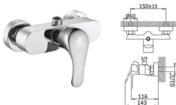
Monomando toma superior 3/4 para kit ducha. Single lever 3/4 upper intake for shower kit
