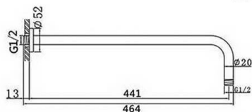
Braço de ducha mural redondo. Round wall shower arm.
