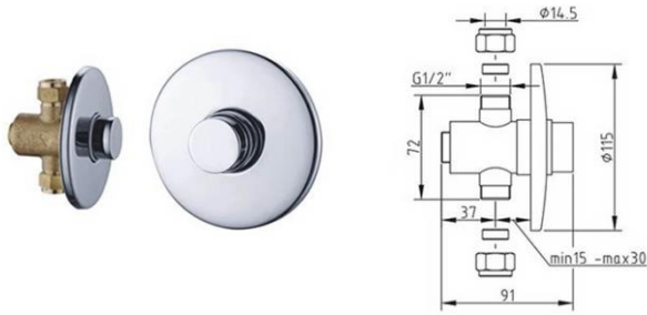
Ducha temporizada para empotrar. Built-in timer shower mixer. Flow duration: 8-12 seconds.
