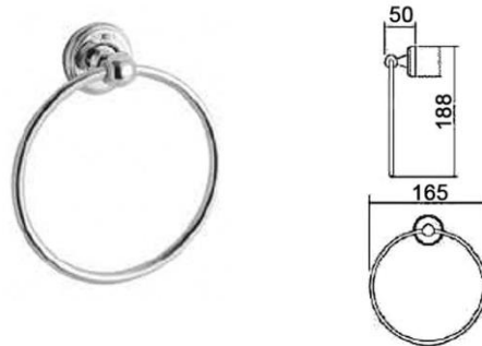
Toallero anilla 25 x 1 mm. Ring towel holder 25 x 1 mm.
